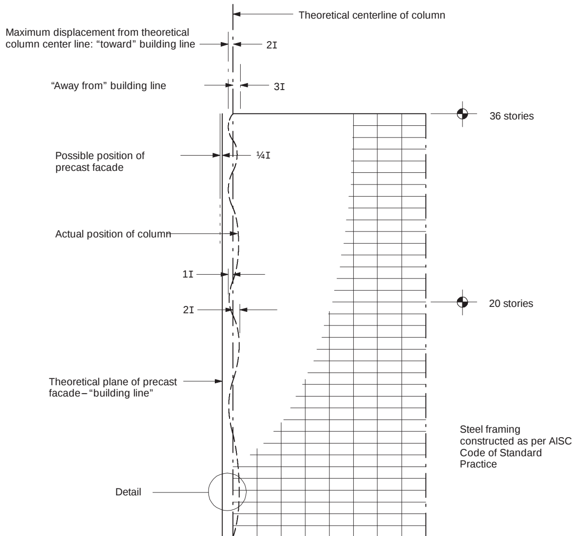
Fig. 14.12.1 Determinate of cladding connection tolerances—high rise steel frame (Example 14.12)
