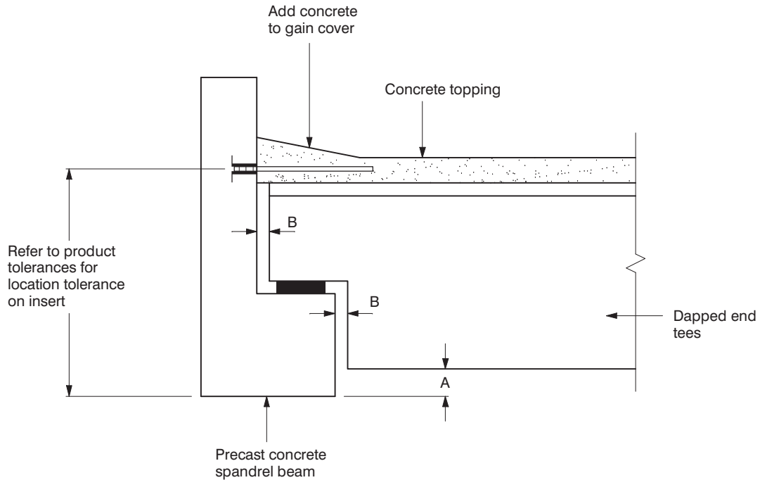
Fig 18.8.1 Detailing Suggestion for Exterior Spandrel Beam to Double Tee Connection
