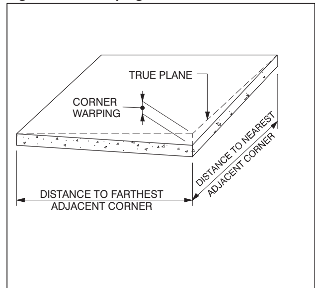
Fig. 8.17.1 Warping Definitions for Panels
