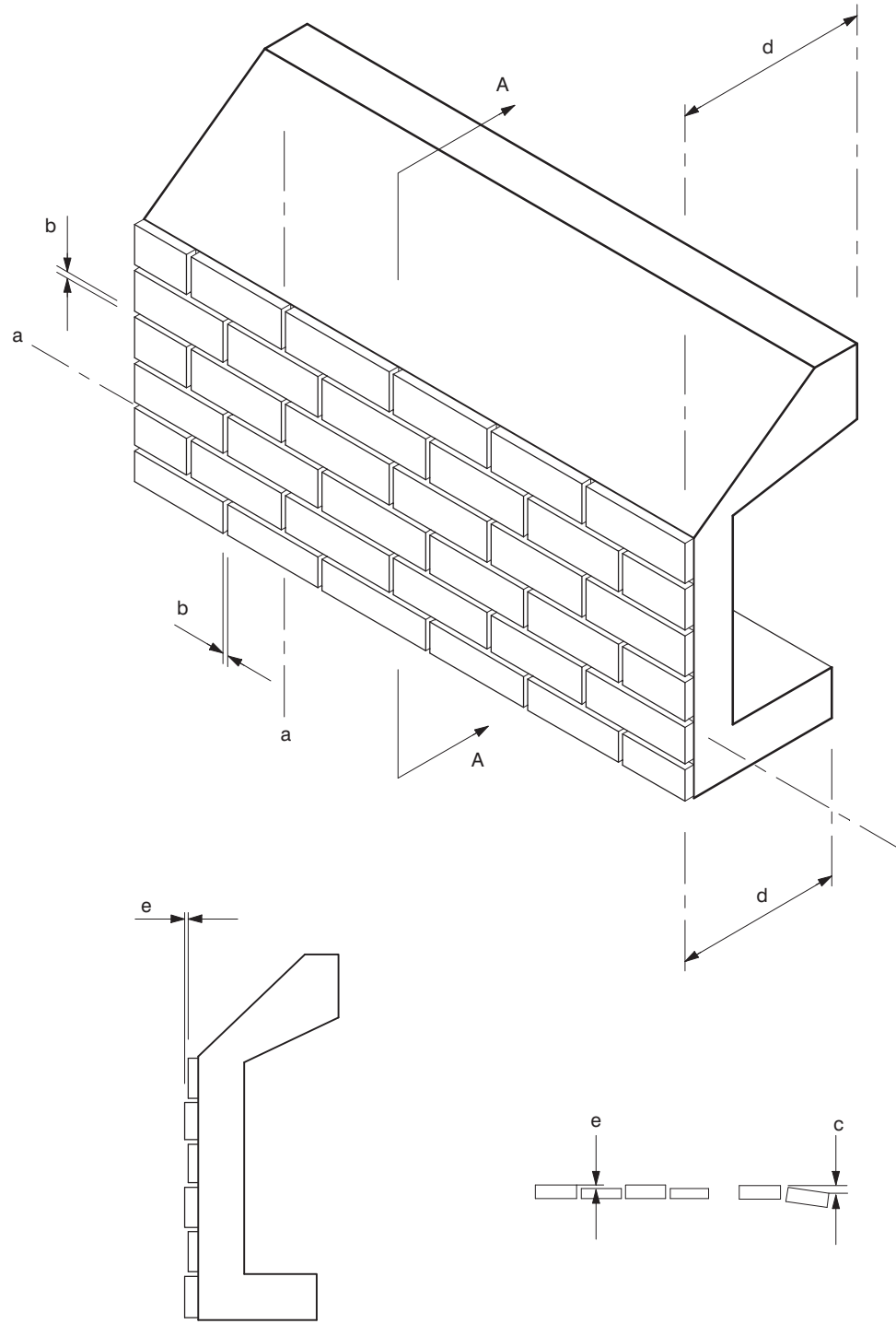
Fig. 10.5.1 Brick Faced Architectural Elements
