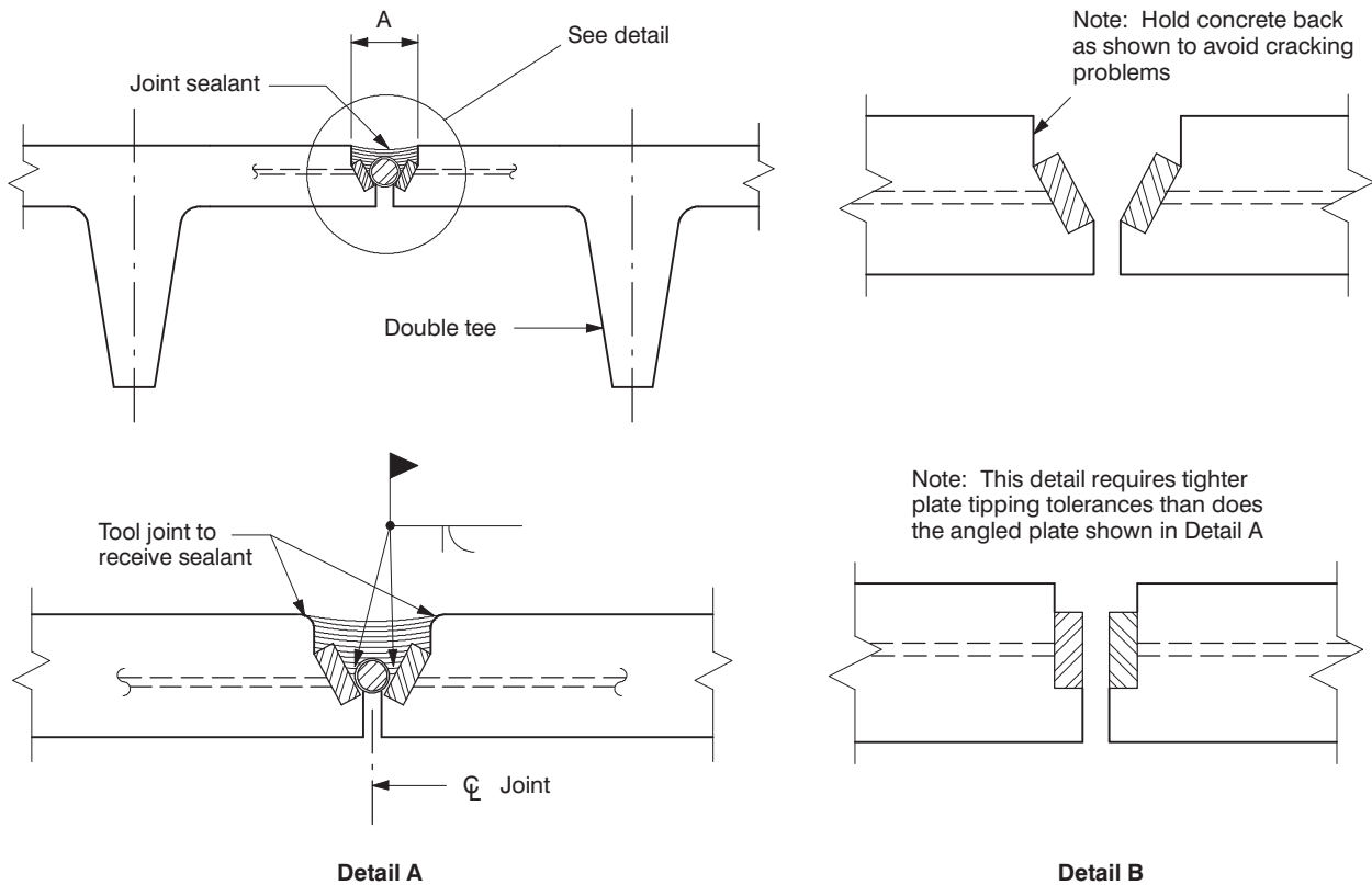
Fig. 18.17.1 Typical Pretopped Double Tee Joints for Parking Structures
