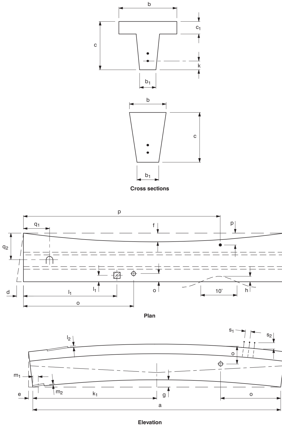
Fig. 10.15.1 Tee Joists/Keystone Joists
