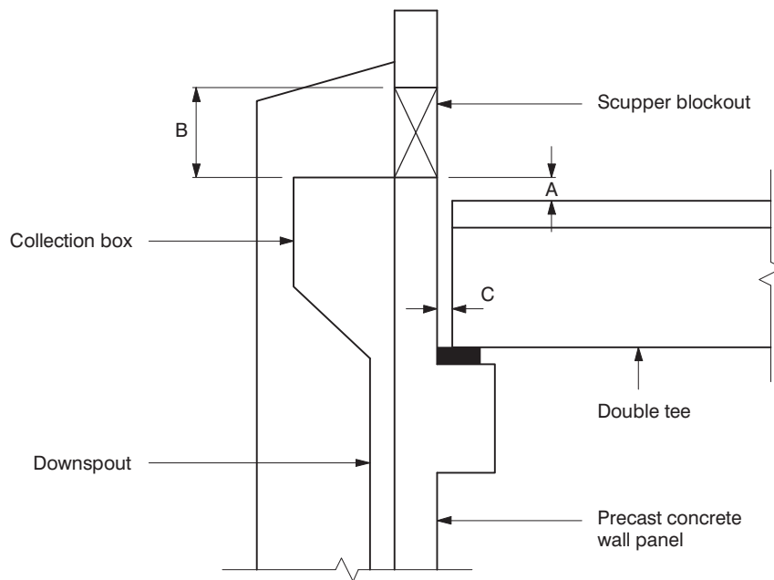
Fig. 18.12.1 Scupper Blockout in Wall Panels
