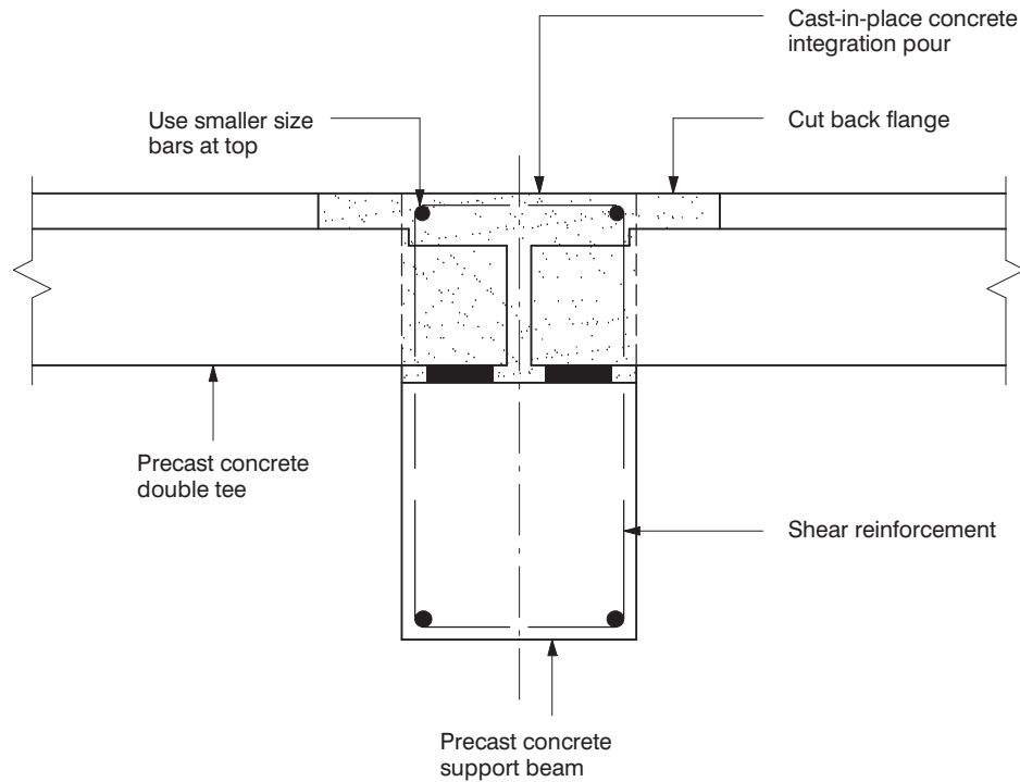
Fig 18.6.1 Detailing Suggestion for Composite Beam Supporting Double Tees
