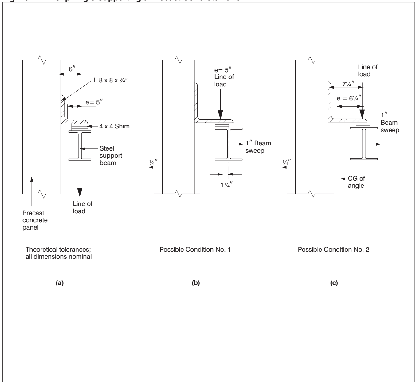
Fig. 19.2.1 Clip Angle Supporting a Precast Concrete Panel
