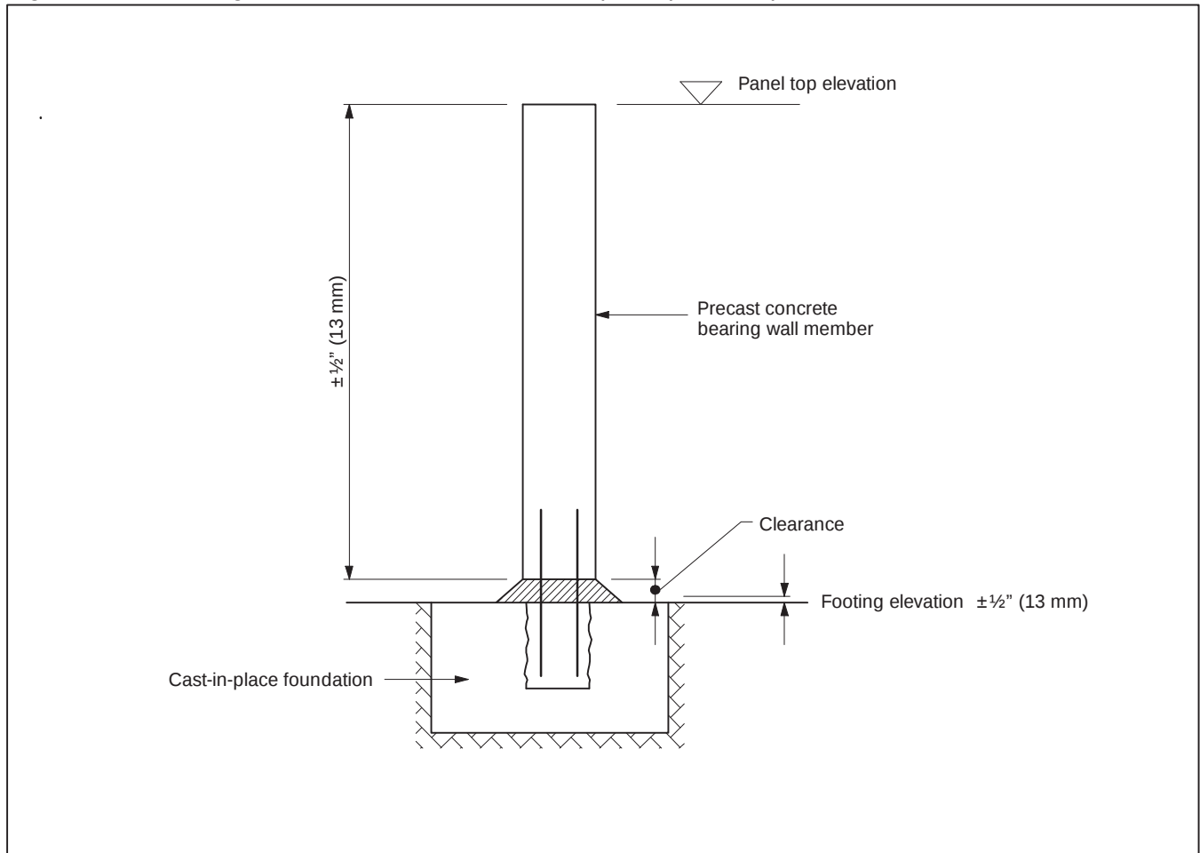
Fig. 14.11.1 Bearing Wall Clearance Determination (Example 14.11)
