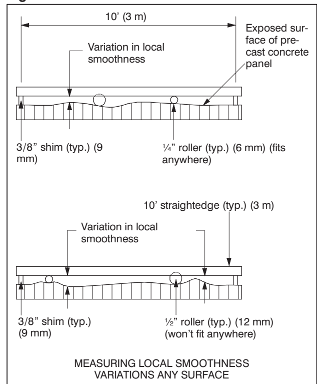
Fig. 8.17.4 Local Smoothness Variations
