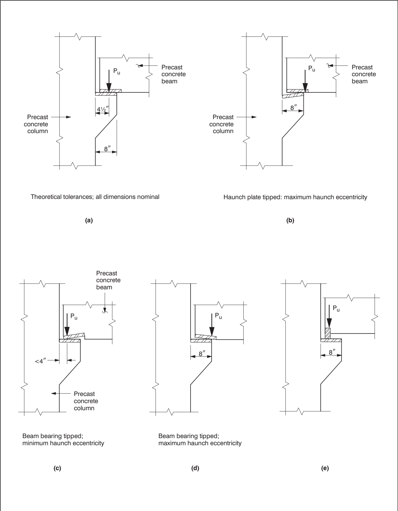
Fig 19.3.1 Precast Corbel with Bearing
