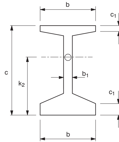
Cross section
