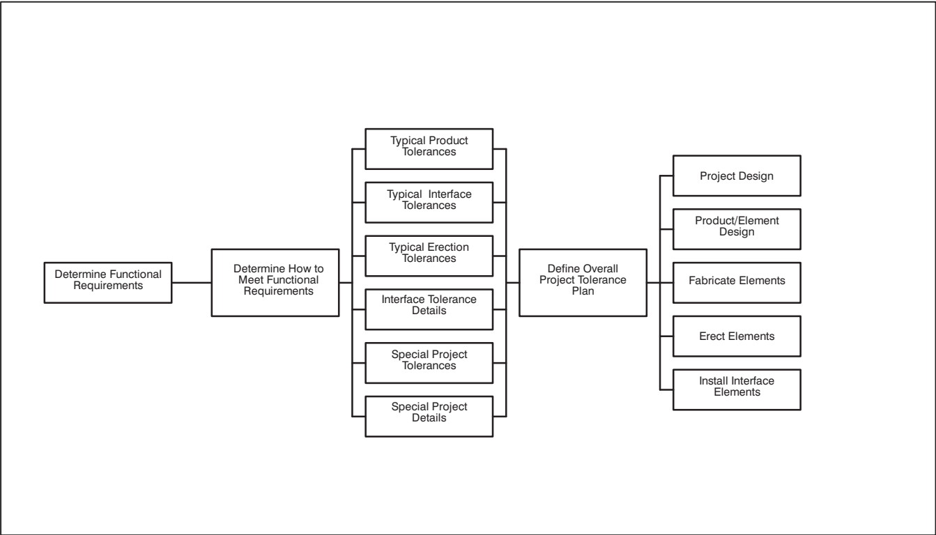
Fig. 1.4.1 Relationship of Project Tolerances to Functional Requirements
