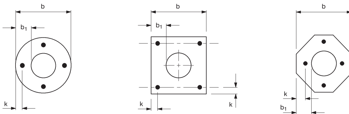
Cross sections
