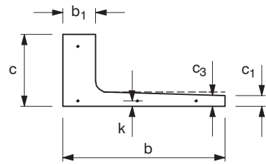
Single riser section
