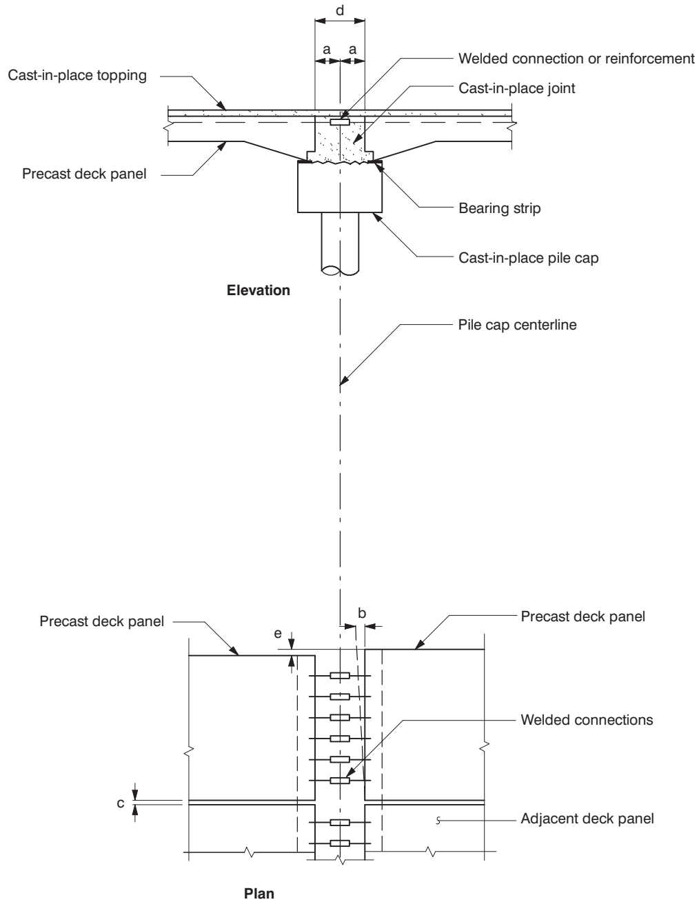
Fig 12.11.1 Pier Deck Erection Tolerances
