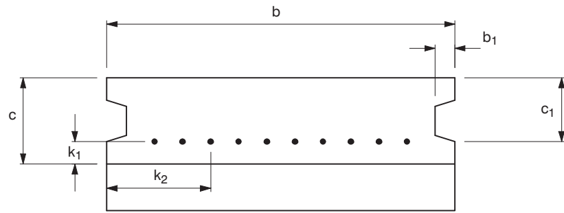
Cross section at midspan
