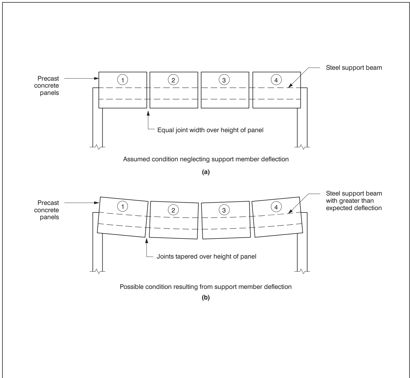
Fig. 19.6.1 Deflection of Supporting Elements
