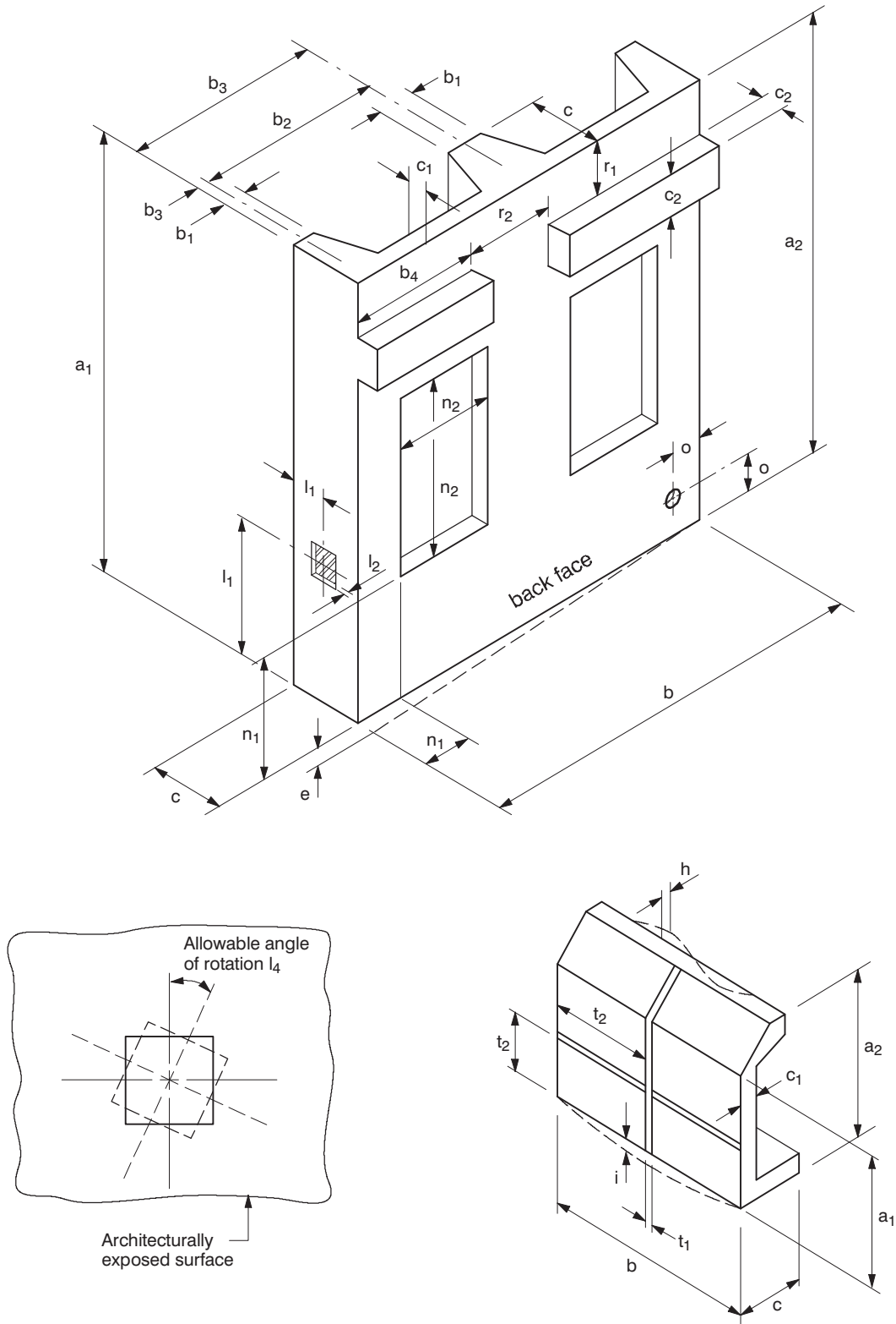
Architectural panels
