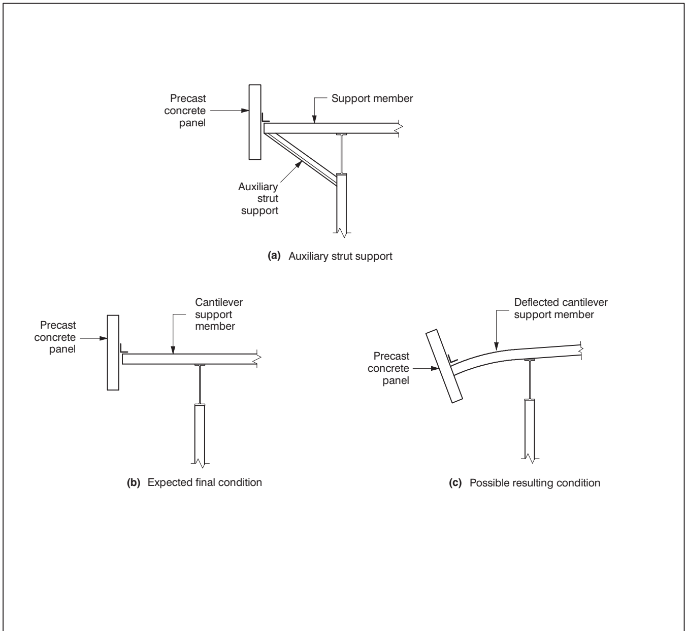
Fig. 19.7.1 Panel Supported by Cantilever
