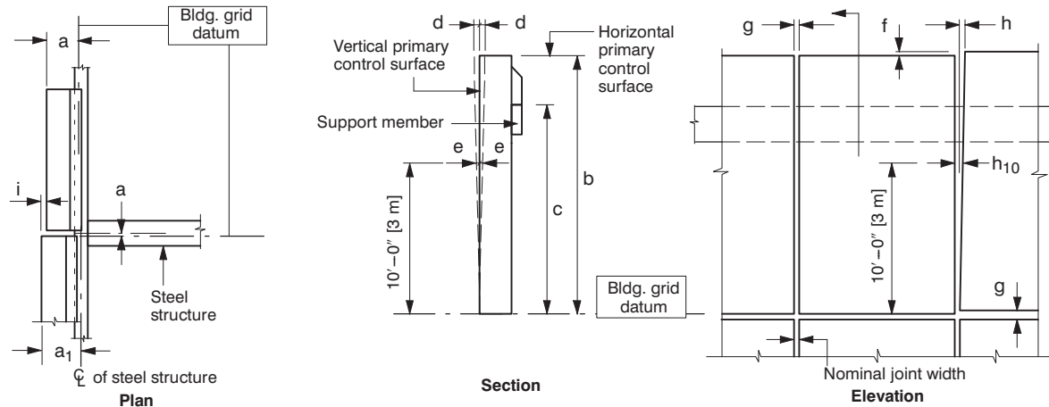
Precast element to structural steel
