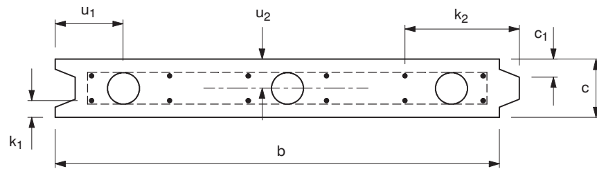
Section
