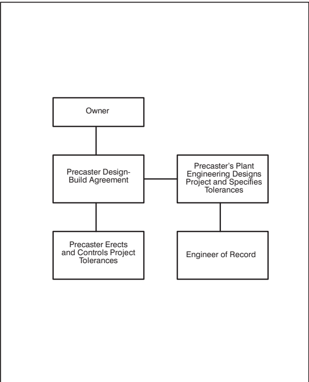
Fig. 1.4.2 Specifying Tolerances—Precaster Design-Build Contract
