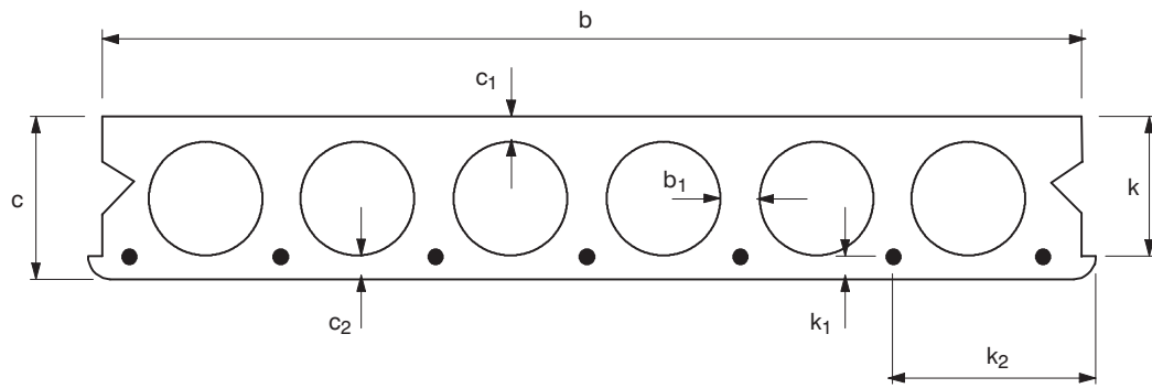
Cross section
