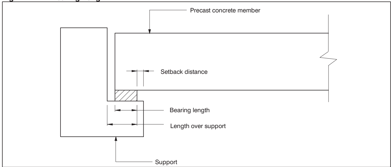
Fig. 11.2.1 Bearing Length
