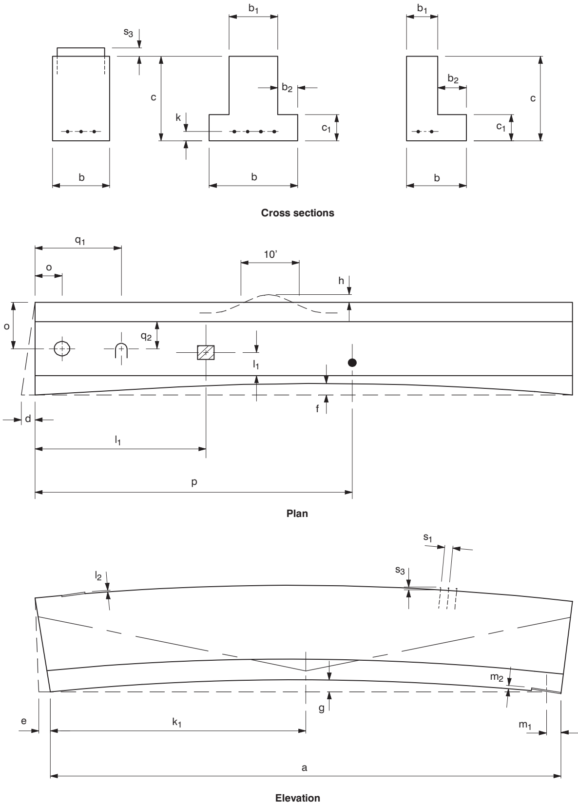
Fig. 10.9.1 Building Beams and Spandrel Beams
