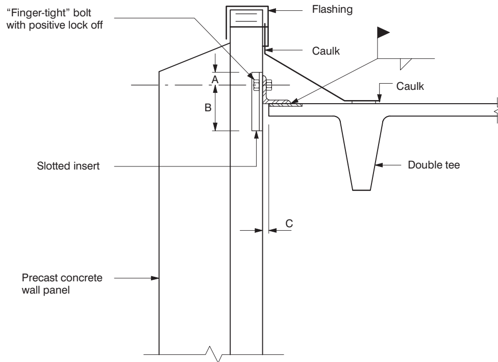
Fig 18.10.1 Wall Panel to Tee Flange Connection
