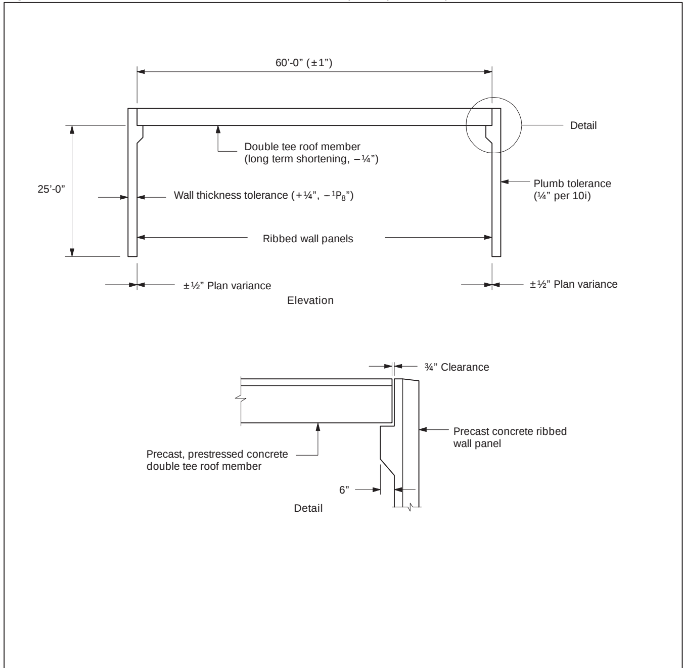
Fig. 14.10.1 Roof Member Clearance Determination (Example 14.10)
