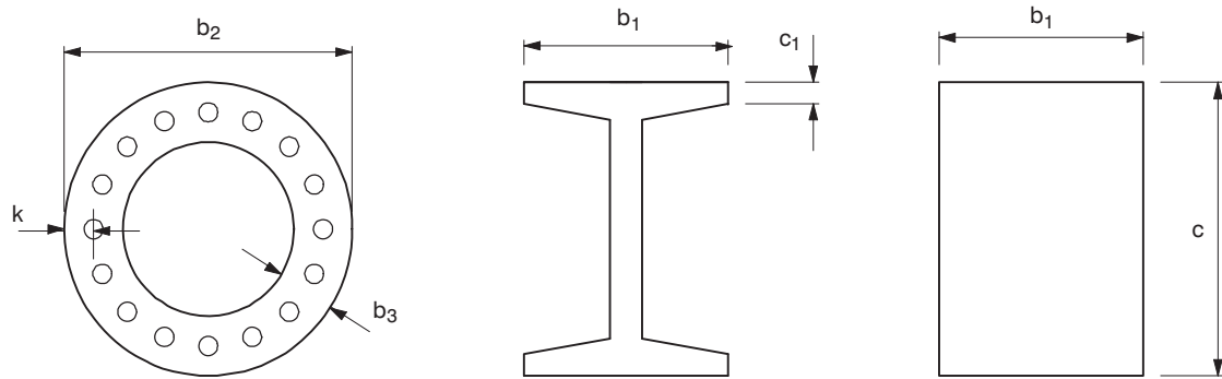
Sections
