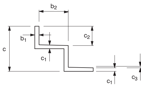
Multi-riser section A
