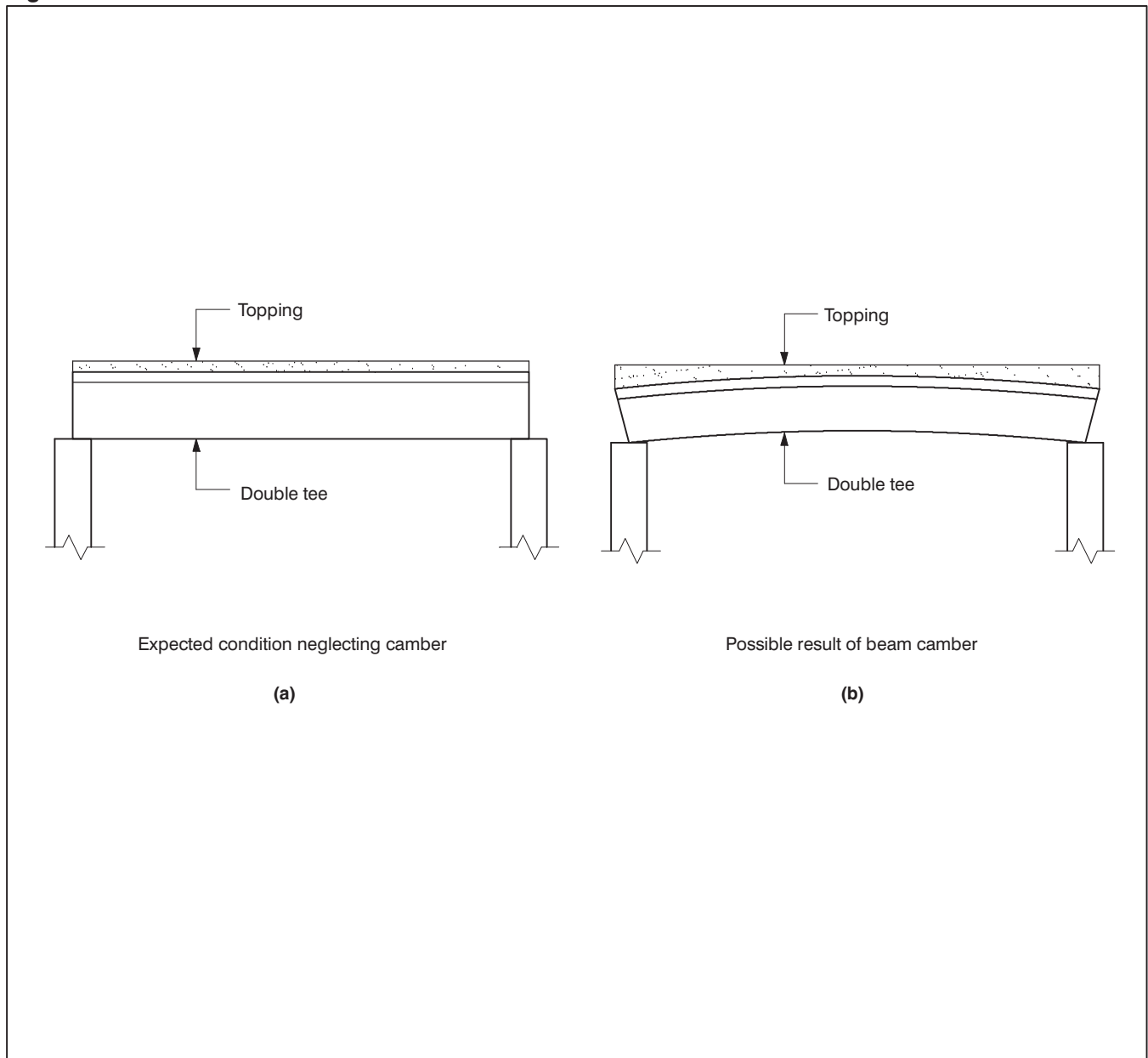
Fig. 19.4.1 Effect of Beam Camber
