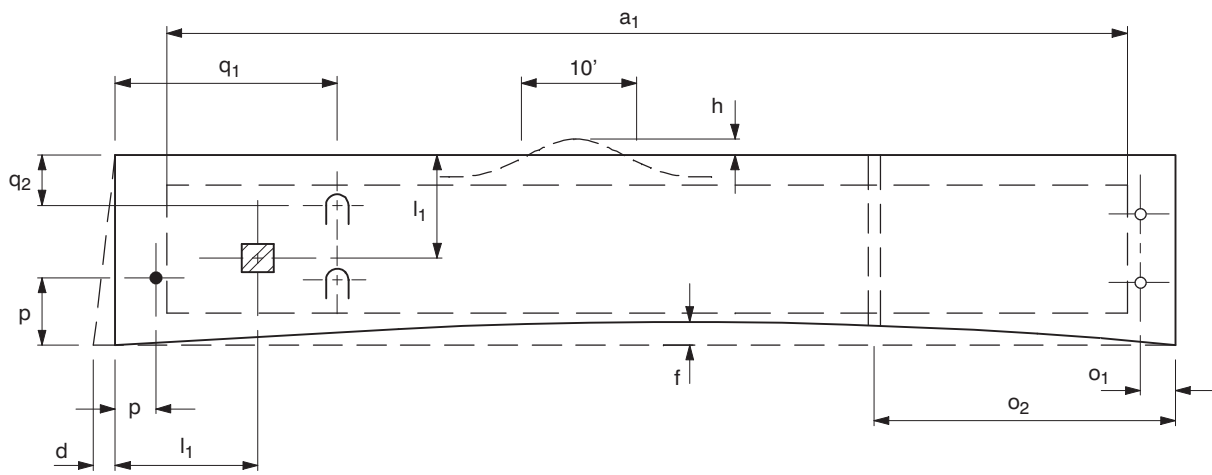
Plan
