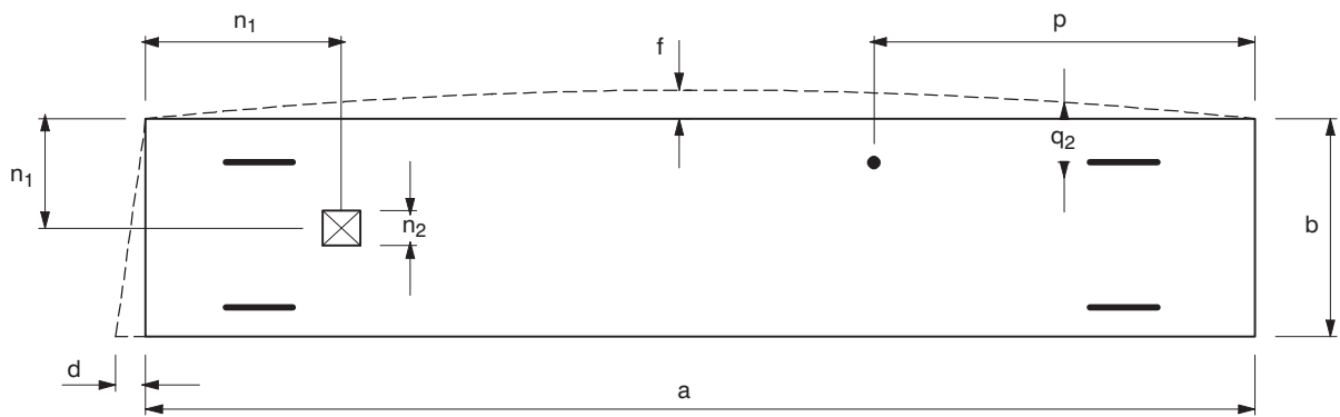
Plan
