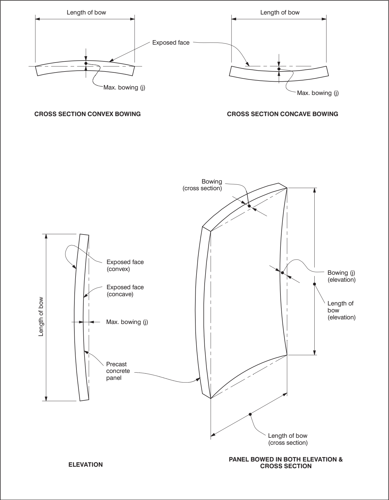
Fig. 8.17.2 Definition of Bowing for Panels
