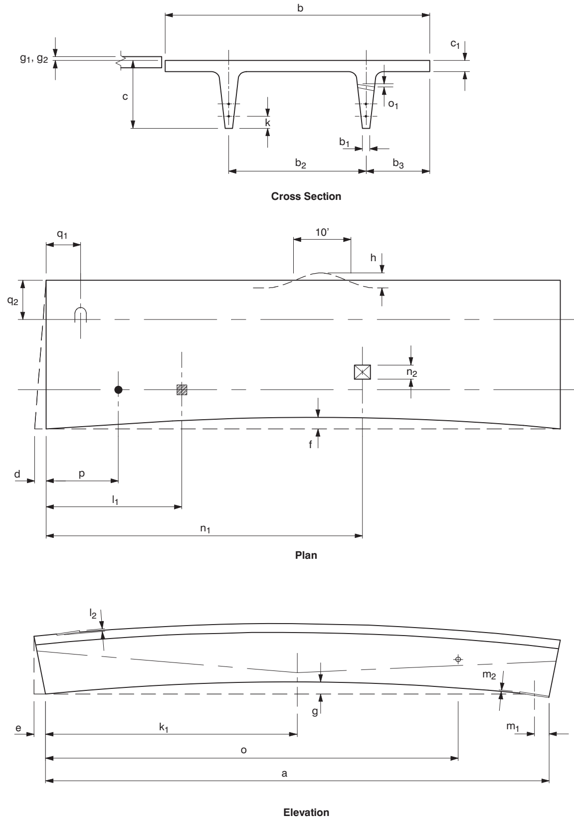
Fig. 10.6.1 Double Tees (Untopped & Pretopped)
