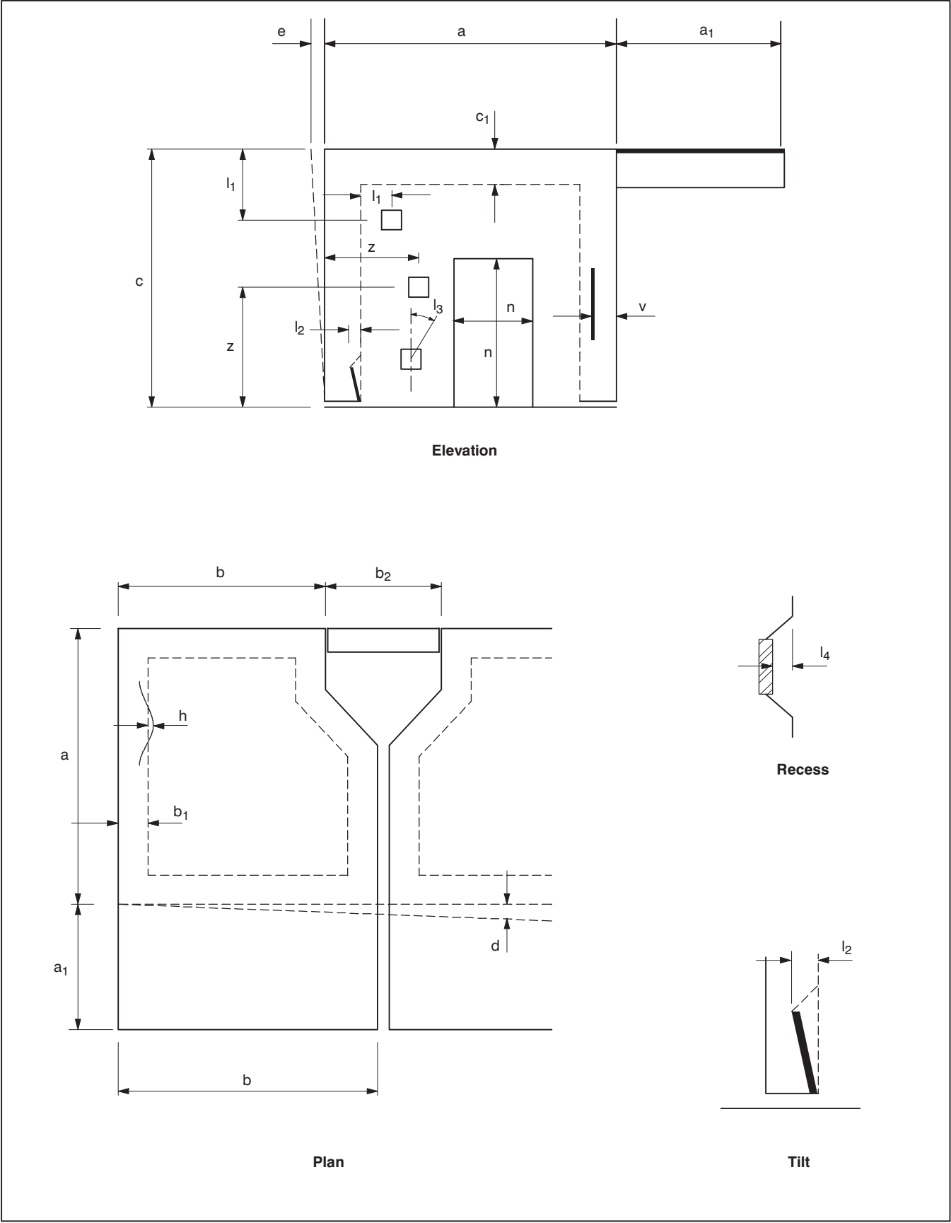
Fig. 10.20.1 Modular Room Unit
