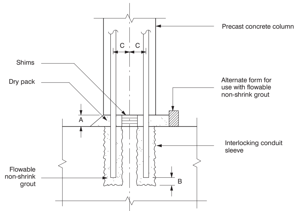
Fig 18.2.1 Detailing Suggestions for Column to Footing Connection Using Footing Sleeves
